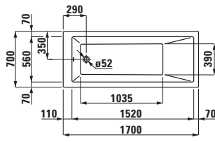
23095.0 Bathtub, drop-in version, sanitary acrylic, 1700x700 mm Badewanne, Einbauversion, Sanitäracryl, 1700x700 mm Baignoire, version encastrée, acrylique sanitaire, 1700x700 mm Vasca, versione da incasso, in acrilico sanitario, 1700x700 mm
