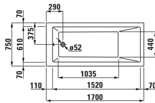
23195.0 Bathtub, drop-in version, sanitary acrylic, 1700x750 mm Badewanne, Einbauversion, Sanitäracryl, 1700x750 mm Baignoire, version encastrée, acrylique sanitaire, 1700x750 mm Vasca, versione da incasso, in acrilico sanitario, 1700x750 mm
