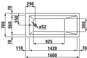
23395.0 Bathtub, drop-in version, sanitary acrylic, 1600x700 mm Badewanne, Einbauversion, Sanitäracryl, 1600x700 mm Baignoire, version encastrée, acrylique sanitaire, 1600x700 mm Vasca, versione da incasso, in acrilico sanitario, 1600x700 mm
