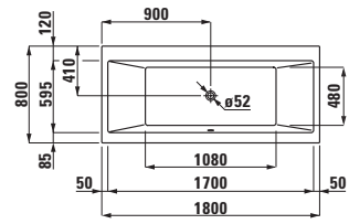
23295.0 Bathtub, drop-in version, sanitary acrylic, 1800x800 mm Badewanne, Einbauversion, Sanitäracryl, 1800x800 mm Baignoire, version encastrée, acrylique sanitaire, 1800x800 mm Vasca, versione da incasso, in acrilico sanitario, 1800x800 mm
